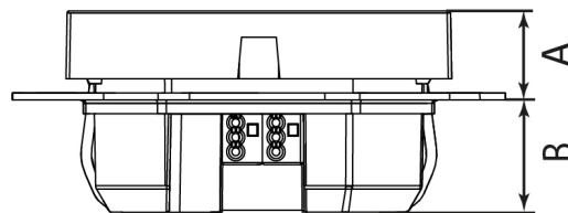
Figure 5: Installation dimensions
