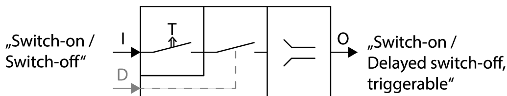
Figure 34: "Staircase function" diagram
