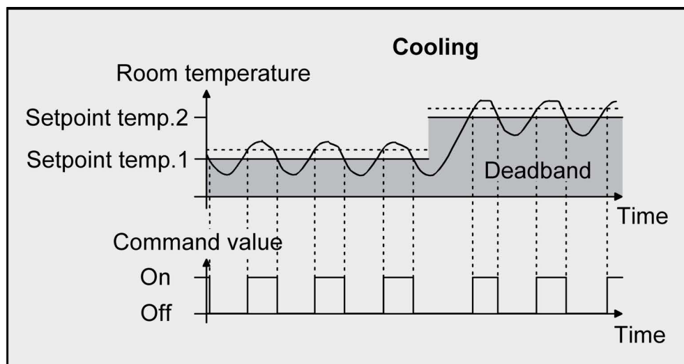
Bild 37: 2-point control for the mixed operating mode of "Heating and cooling" in active cooling mode
