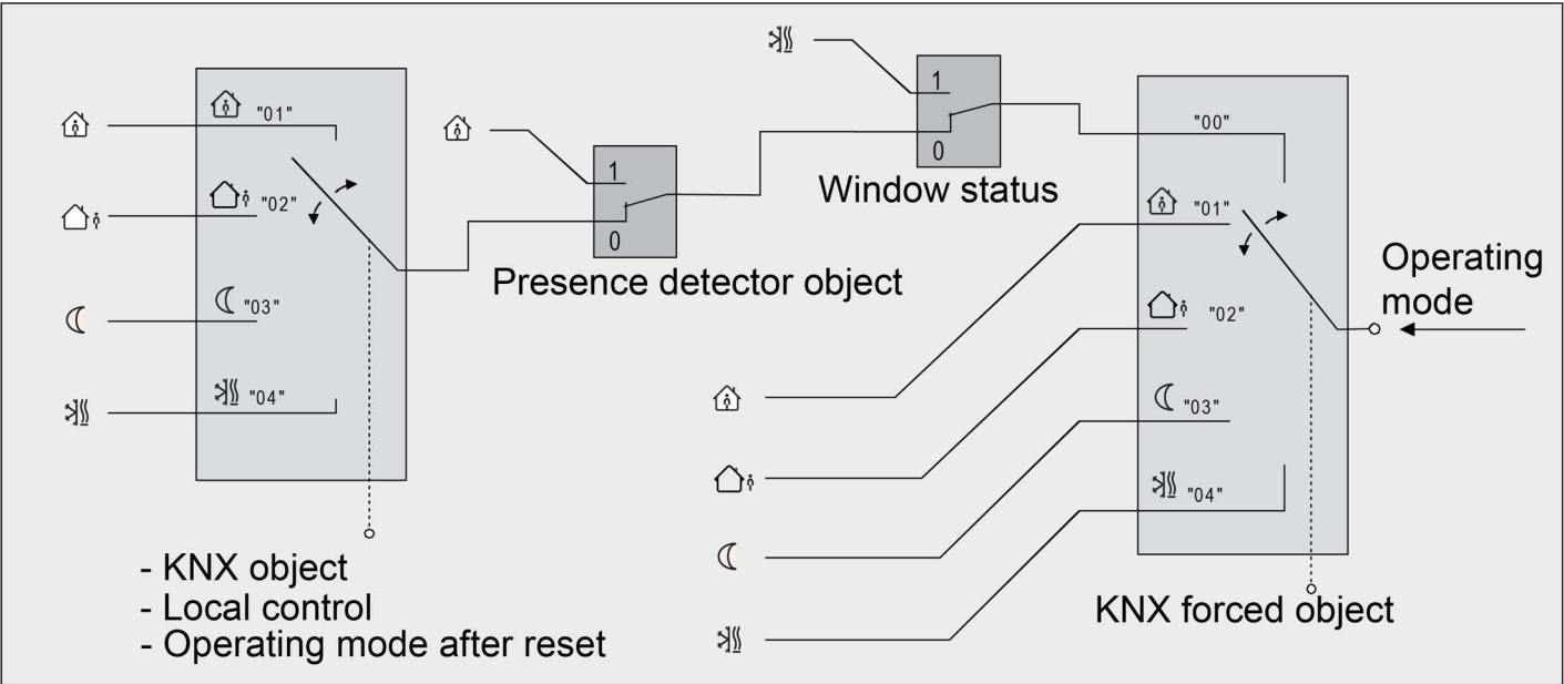
Bild 41: Operating mode changeover by KNX object with presence detector
