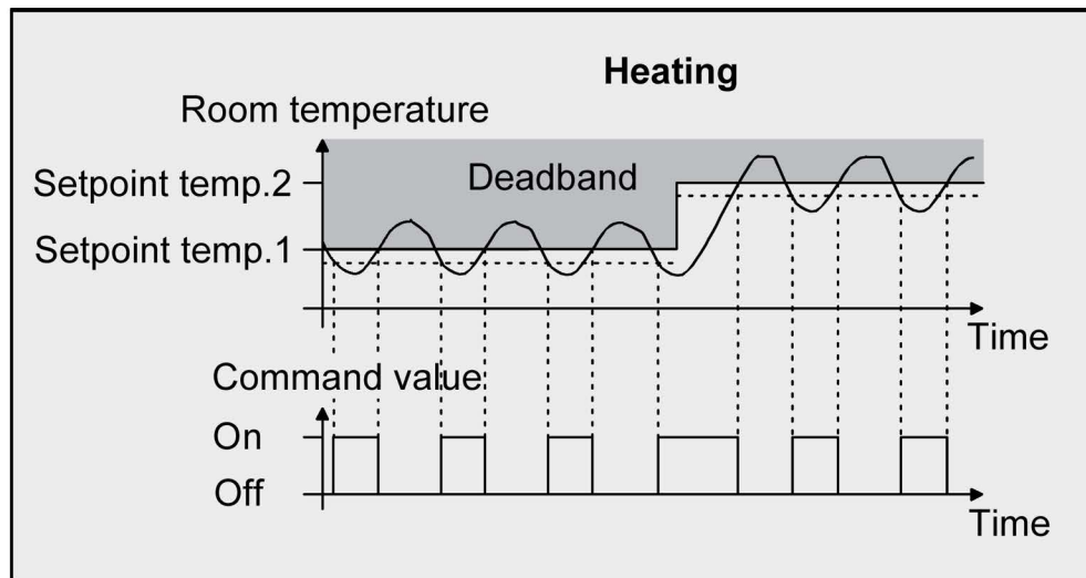
Bild 36: 2-point control for the mixed operating mode of "Heating and cooling" in active heating mode
