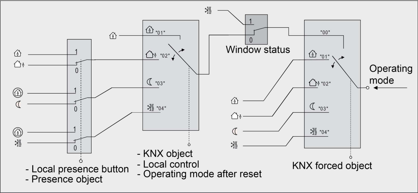
Bild 40: Operating mode changeover by KNX object with presence button
