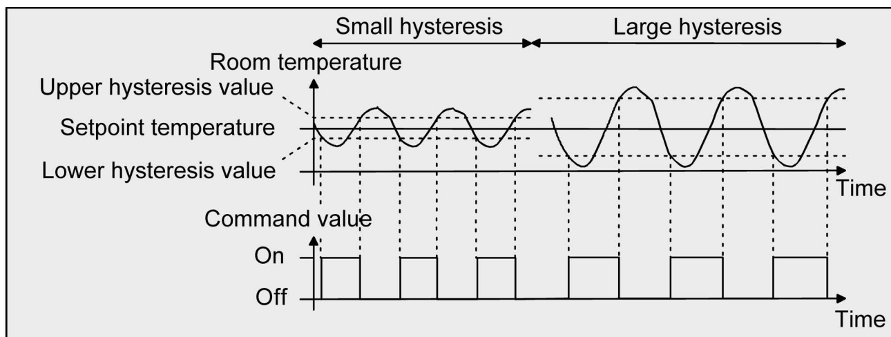
Bild 39: Effects of the hysteresis on the switching behaviour of the variable of a 2-point control
