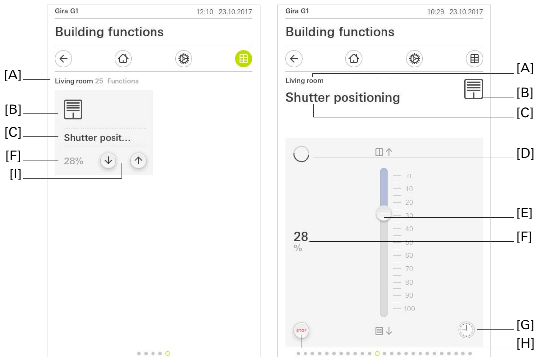
Bild 15: Example of operating and display element of the "Shutter position" function
