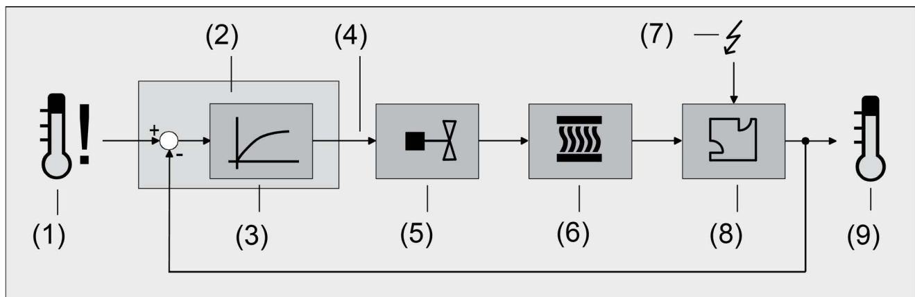
Bild 31: Regulated system of a single-room temperature control
