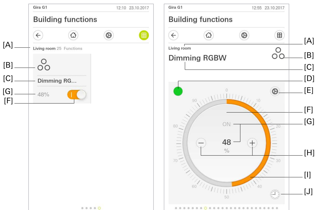
Bild 9: Example of operating and display element of the "Dimming RGBW" function
