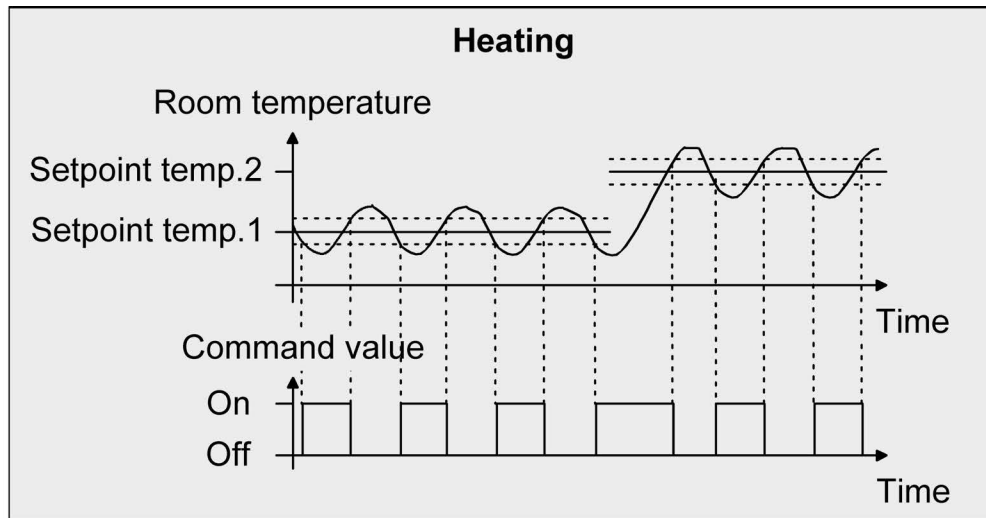
Bild 34: 2-point control for the "Heating" operating mode
