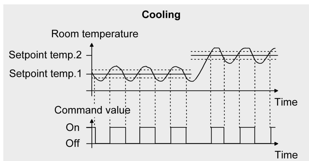
Bild 35: 2-point control for the "Cooling" operating mode
