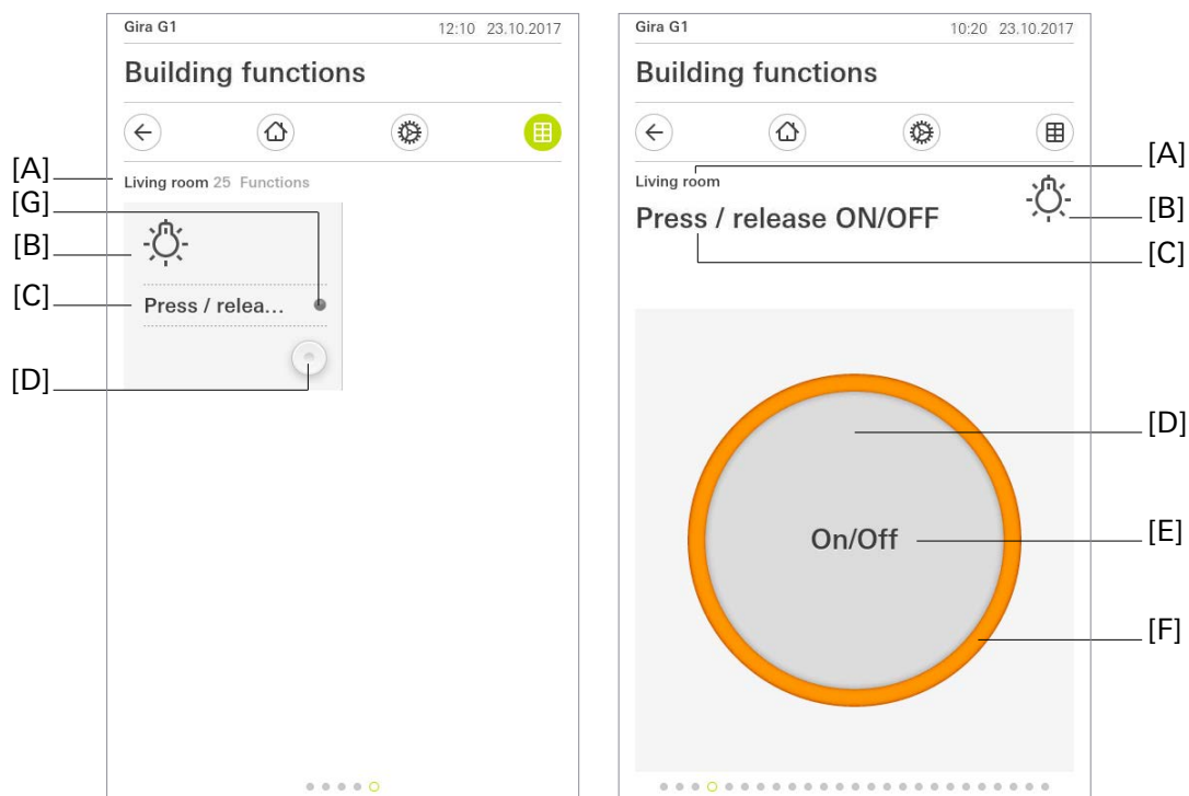
Bild 4: Example of operating and display element of the "Press / release ON/OFF" function
