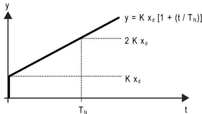
Bild 38: Function of the corrected variable of a PI control
