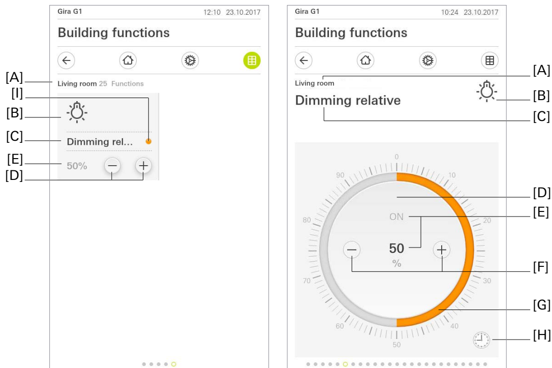
Bild 6: Example of operating and display element of the "Dimming relative" function
