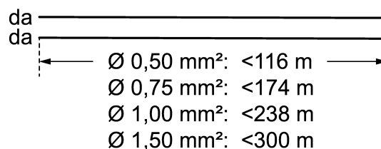
Figure 3: DALI cable length
