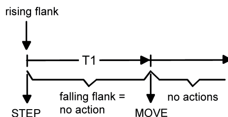
Figure 17: Operation concept "long – short"
