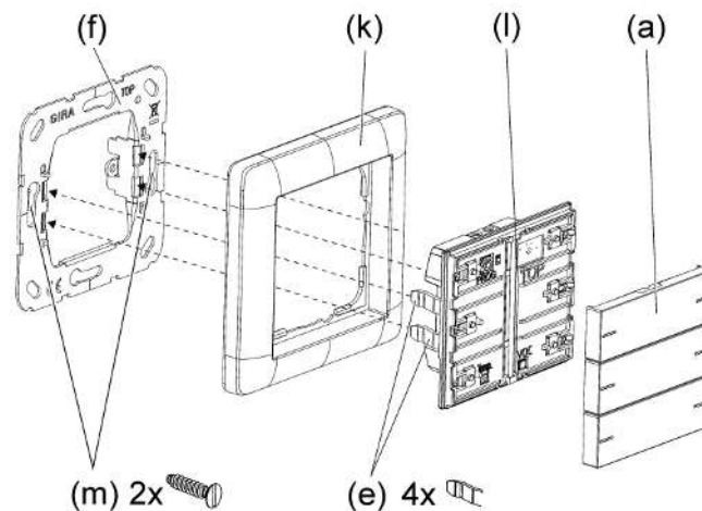
Figure 5: Mount device
