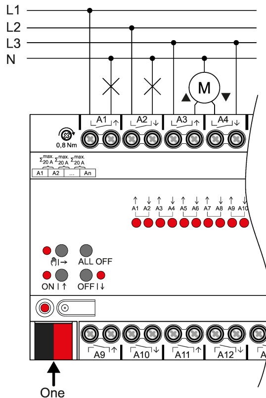
Image 3: Device connection (connection example)
