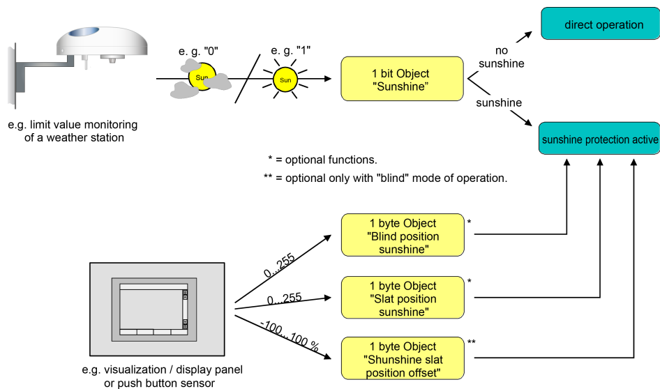
Figure 16: Schematic diagram illustrating the simple sun protection configuration
