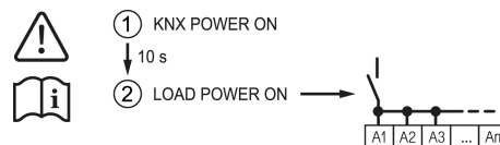
Figure 6: Sequence during commissioning
