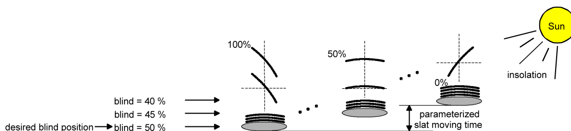
Figure 12: Example of slat positioning affecting the position of the Venetian blind (typical of slat type 1; analogous reaction for type 2)
