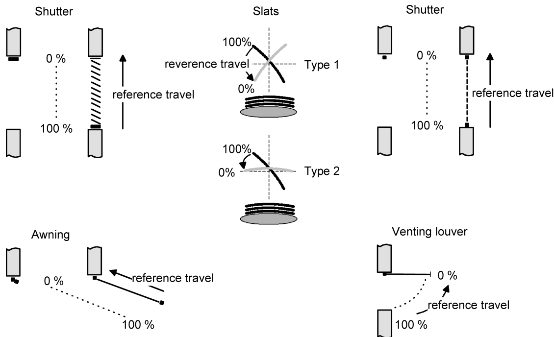
Figure 14: Reference movement
