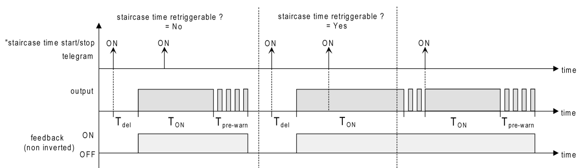
Figure 19: Switch-on behaviour of the staircase function
