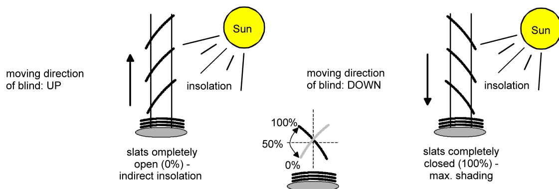
Figure 43: Type 1 - Slatted Venetian blinds with oblique slat position in both travel directions
