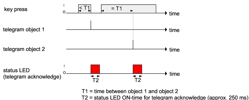
Figure 91: Example of operating concept "Channel 1 or Channel 2"
