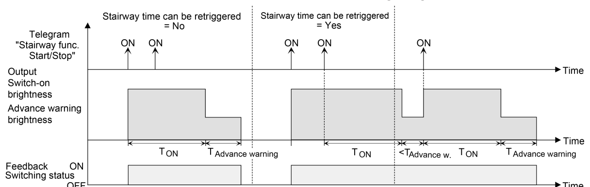
Figure 15: Switch-on behaviour of the staircase function without soft functions
