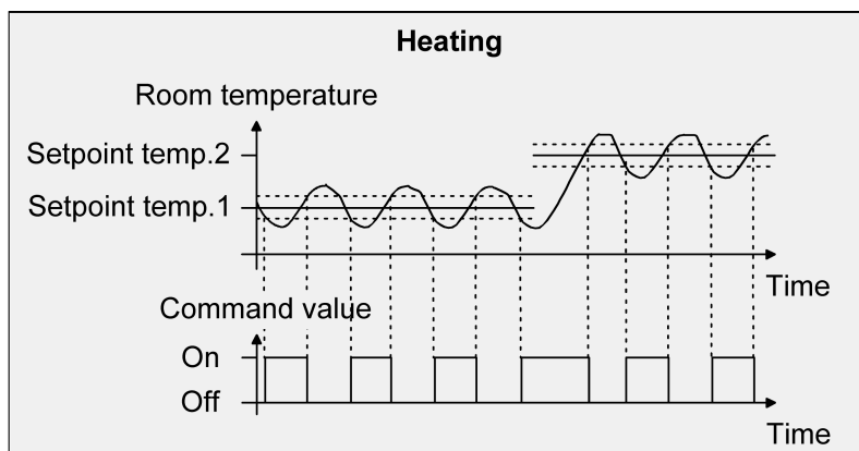
Figure 70: 2-point feedback control for the single "Heating" operating mode
