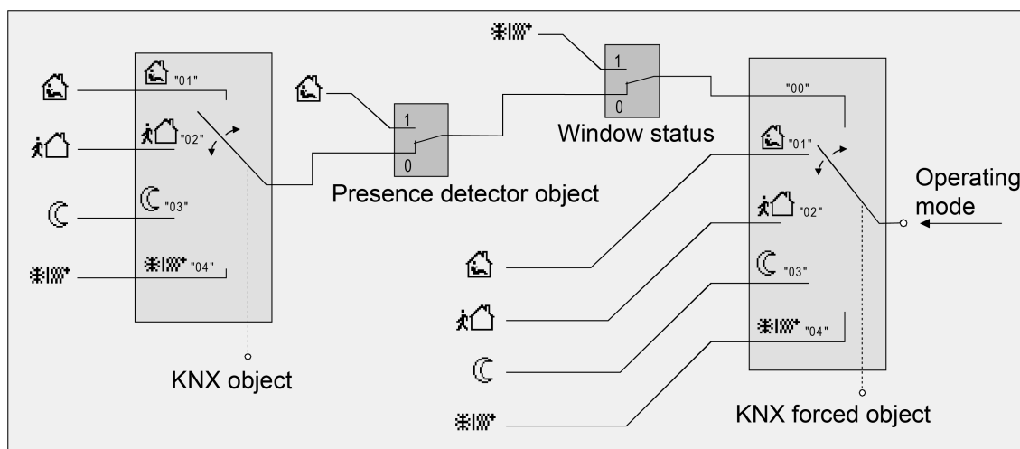
Figure 76: Operating mode switchover through KNX object with presence detector
