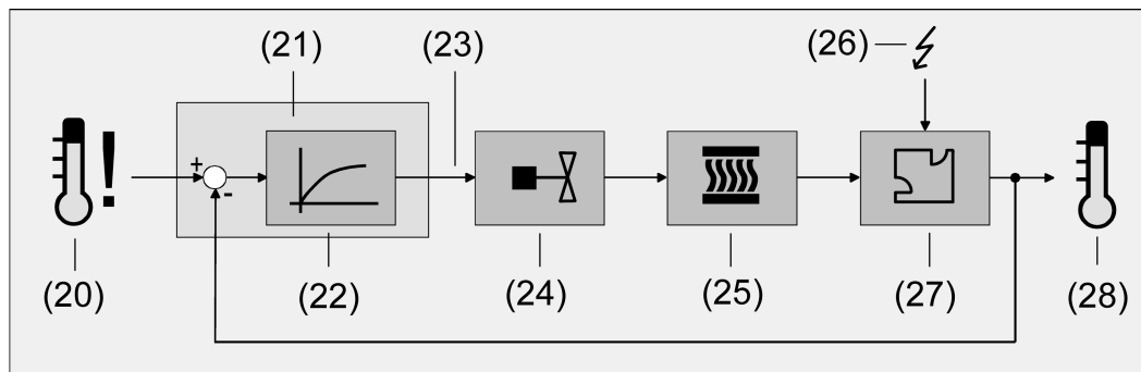
Figure 67: Controlled system of single-room temperature control
