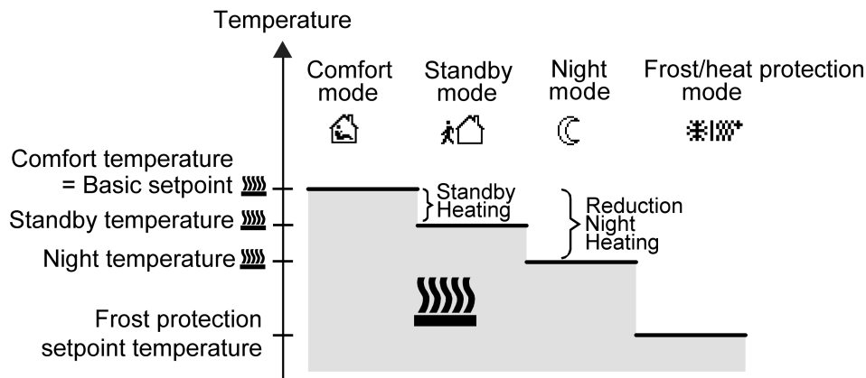
Figure 77: Setpoint temperatures in the operating mode "Heating"
