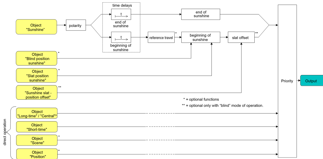
Figure 51: Function diagram illustrating the sun protection
