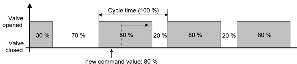
Figure 60: Example of a command value change 30% -> 80% during the opening phase of the valve
