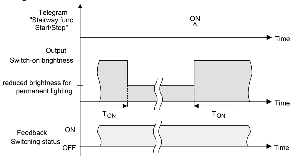
Figure 21: The continuous lighting of the staircase function without soft functions
