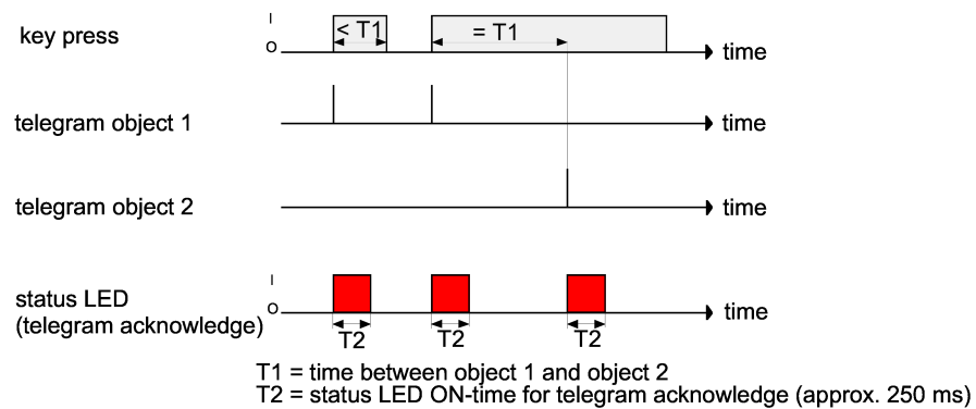
Figure 92: Example for operating concept "Channel 1 and channel 2"
