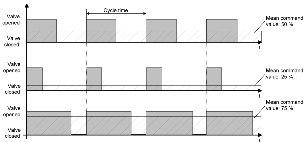
Figure 56: Resulting mean value through variable duty factor with pulse width modulation
