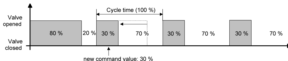
Figure 57: Example of a command value change 80% -> 30% during the opening phase of the valve
