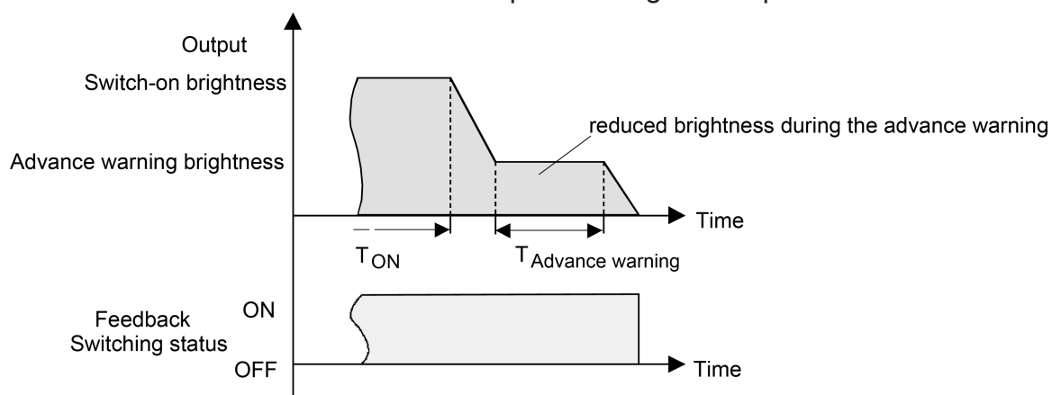
Figure 39: The pre-warning function of the staircase function with soft OFF function (as an example with minimum brightness = 0%)
