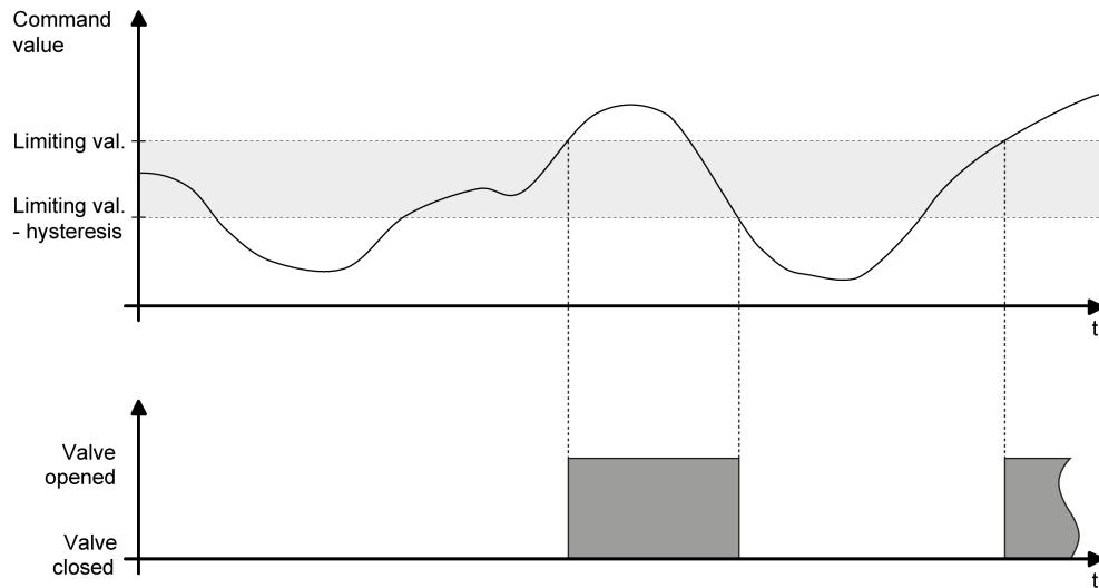
Figure 63: Example of command value evaluation with limiting value
