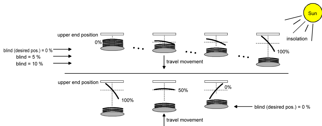
Figure 47: Example of slat positioning with the Venetian blind in upper end position (Typical of slat type 1.)
