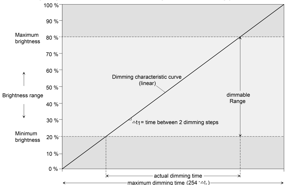
Figure 27: Linear characteristic dimming curve as an example with minimum brightness > 0 % and maximum brightness
