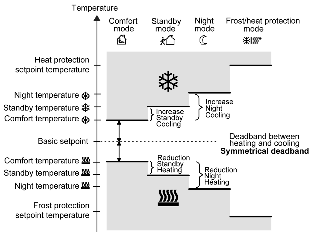
Figure 79: Setpoint temperatures in the operating mode "Heating and cooling" with symmetrical deadband
