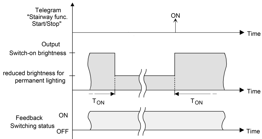
Figure 40: The continuous lighting of the staircase function without soft functions
