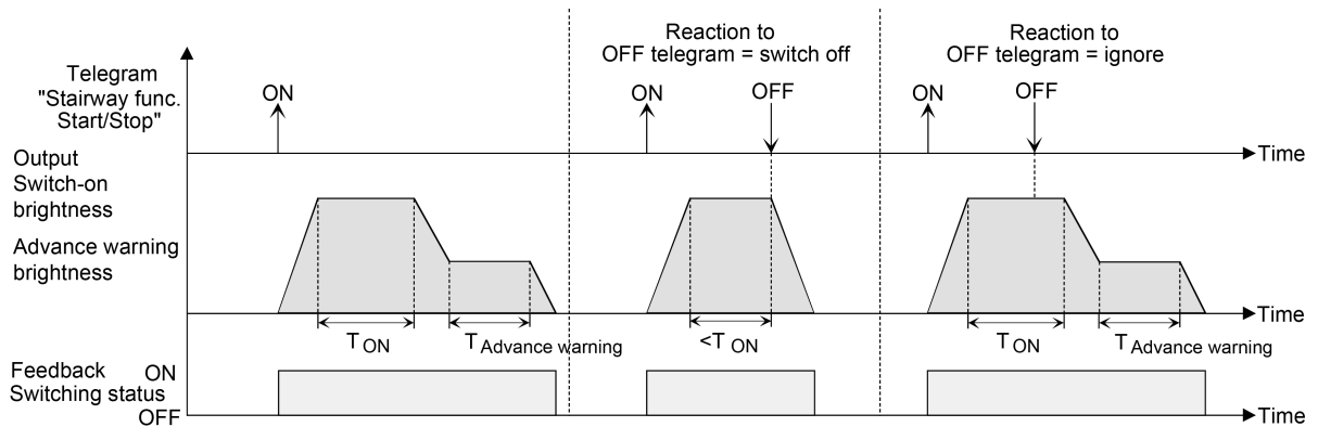
Figure 18: Switch-off behaviour of the staircase function with soft functions (as an example with minimum brightness = 0 %)
