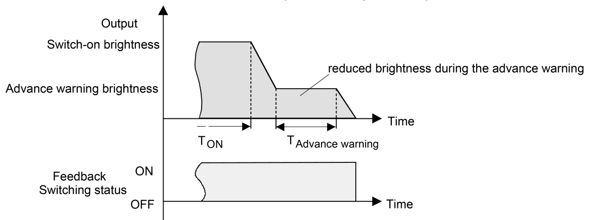
Figure 20: The pre-warning function of the staircase function with soft OFF function (as an example with minimum brightness = 0%)
