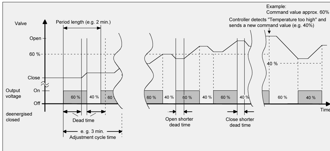
Figure 65: Ideal course of the valve stroke for a Cycle time < Adjusting cycle time
