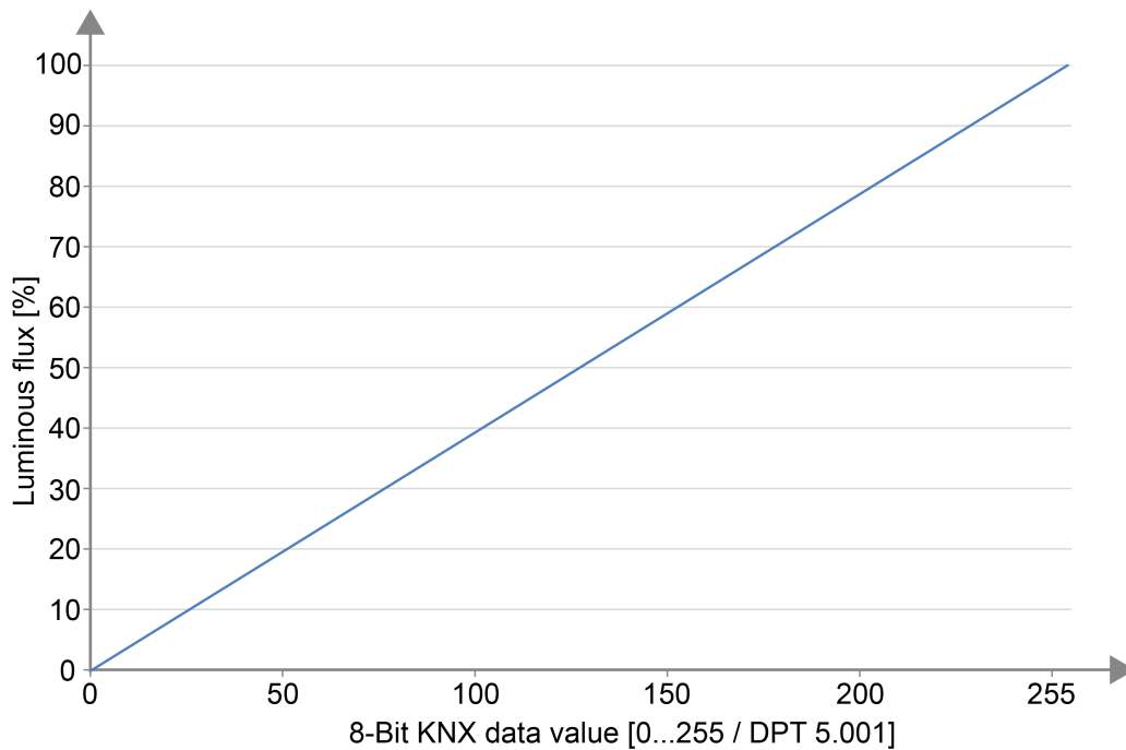
Figure 25: Linear DALI dimming characteristic (relative luminous flux [%] depending on the 8-bit KNX data value [0...255])
