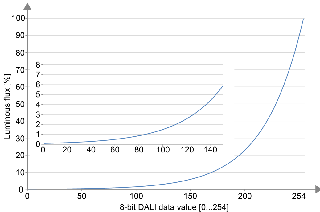
Figure 24: Logarithmic dimming curve in DALI operating devices (relative luminous flux [%] depending on the 8-bit DALI data value [0...254])
