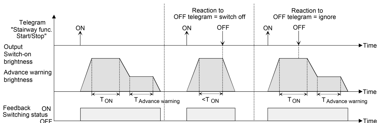
Figure 37: Switch-off behaviour of the staircase function with soft functions (as an example with minimum brightness = 0 %)
