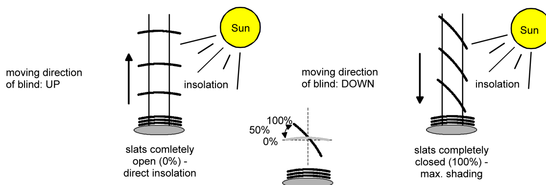
Figure 44: Type 2 - Slatted Venetian blinds with oblique and horizontal slat position
