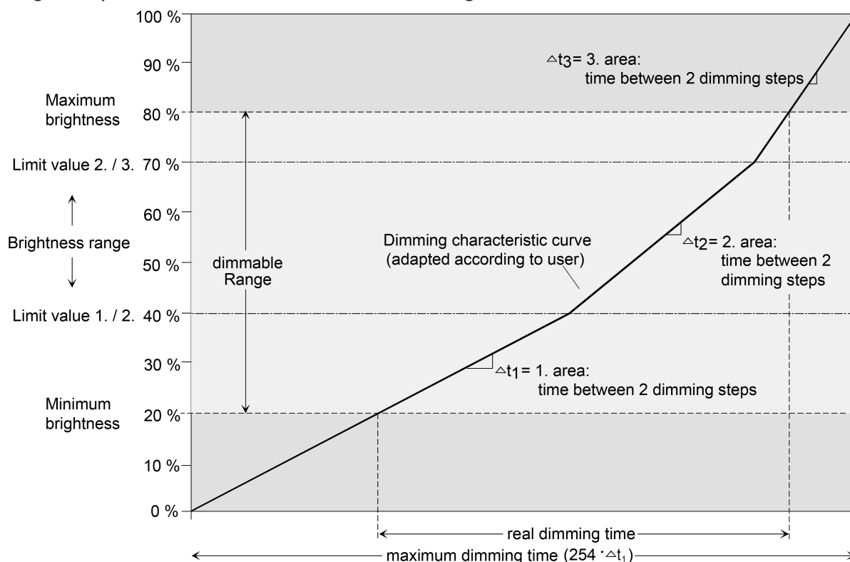
Figure 11: User-defined dimming characteristic as an example with minimum brightness and maximum brightness
