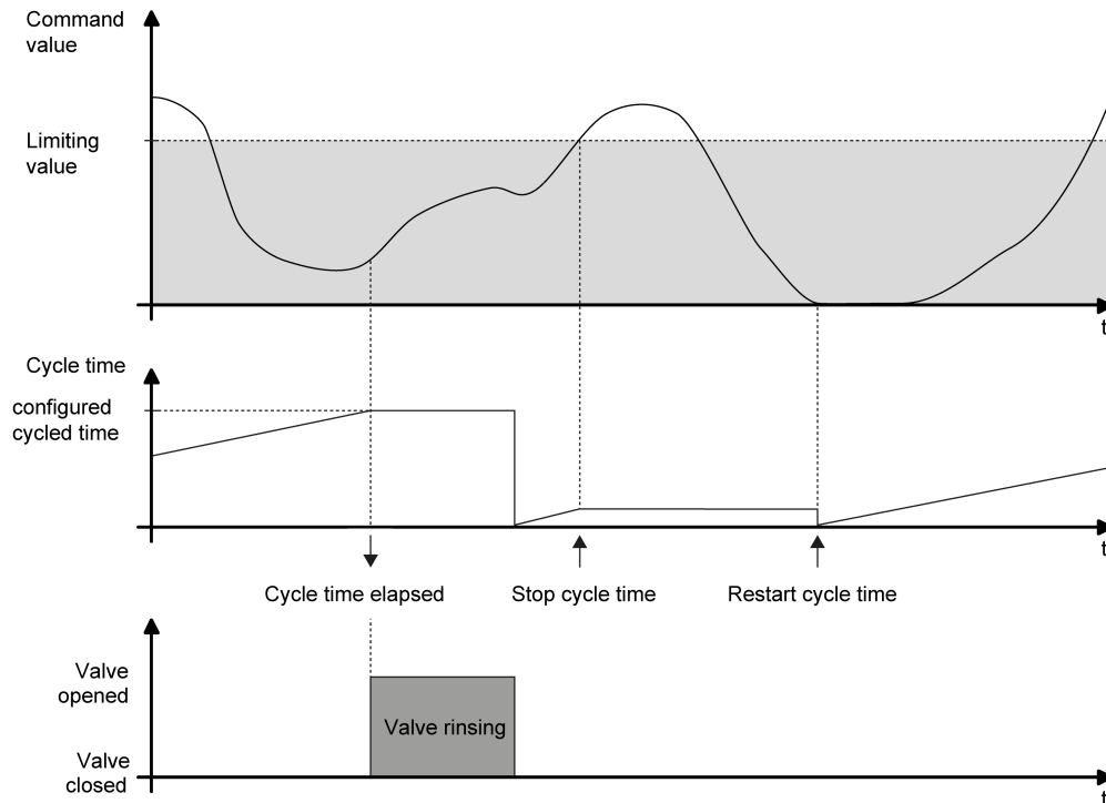
Figure 66: Example of a minimum command value limiting value for intelligent valve rinsing
