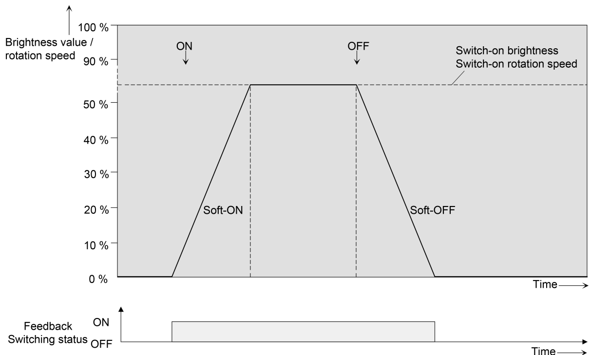
Figure 13: Dimming behaviour of the soft ON/OFF functions (as an example)
