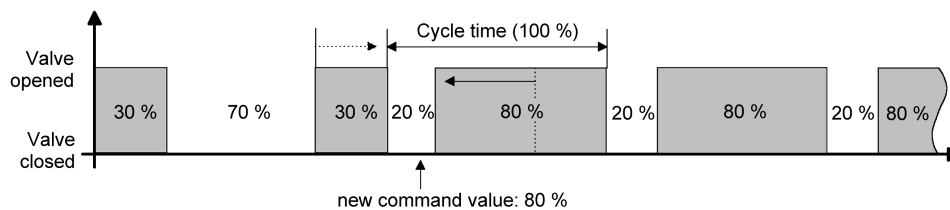
Figure 61: Example of a command value change 30% -> 80% during the closing phase of the valve
