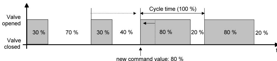
Figure 62: Example of a command value change 30% -> 80% during the opening phase of the valve (opening phase too long)
