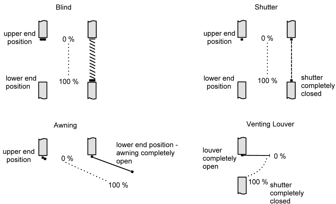
Figure 45: Positions defined as a function of the type of movement
