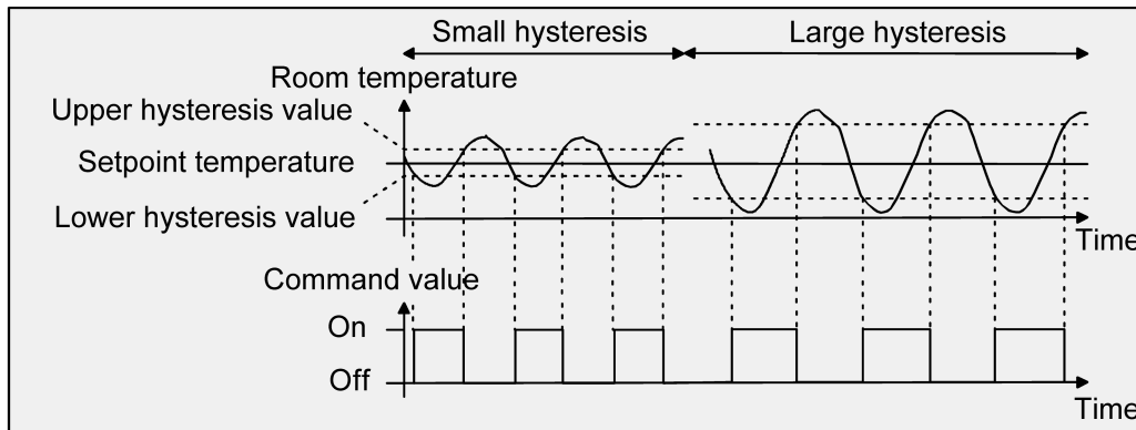
Figure 74: Effects of the hysteresis on the switching behaviour of a 2-point feedback control command value
