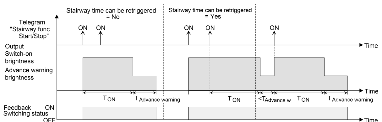
Figure 34: Switch-on behaviour of the staircase function without soft functions
