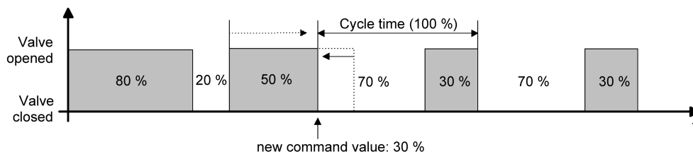
Figure 59: Example of a command value change 80% -> 30% during the opening phase of the valve (opening phase too long)
