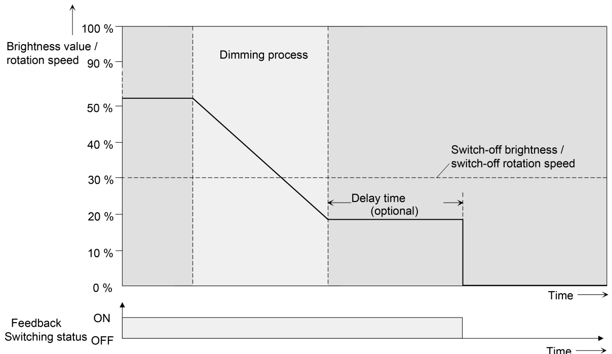
Figure 33: Dimming and switching behaviour of the automatic switch-off function
