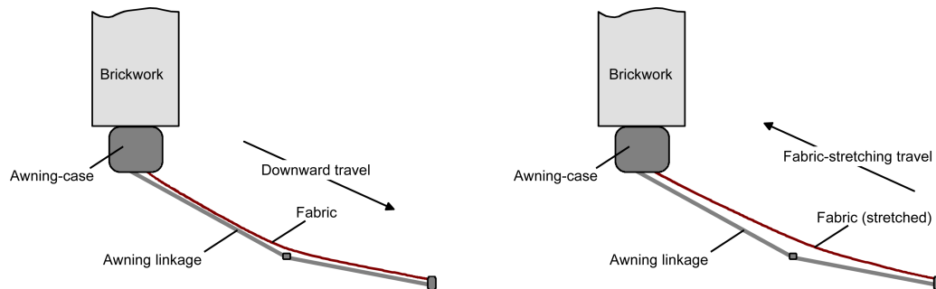
Figure 54: Fabric stretching in an awning
