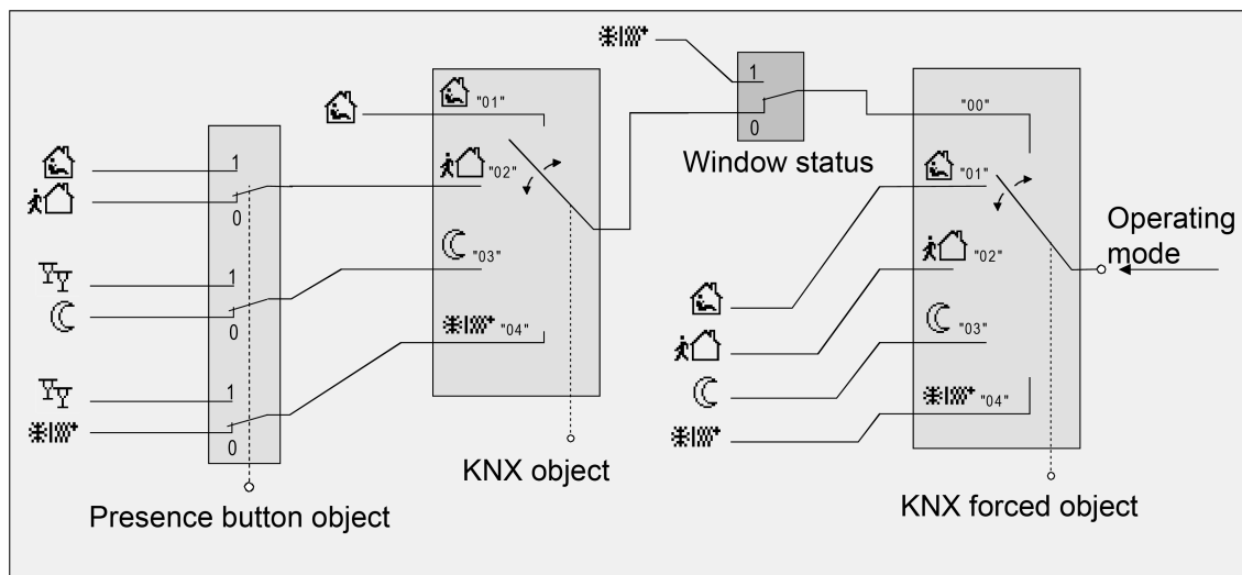
Figure 75: Operating mode switchover through KNX object with presence button
