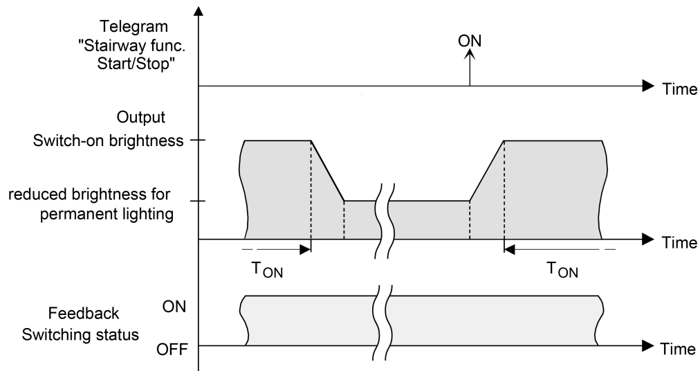
Figure 22: The continuous lighting of the staircase function with soft OFF functions
