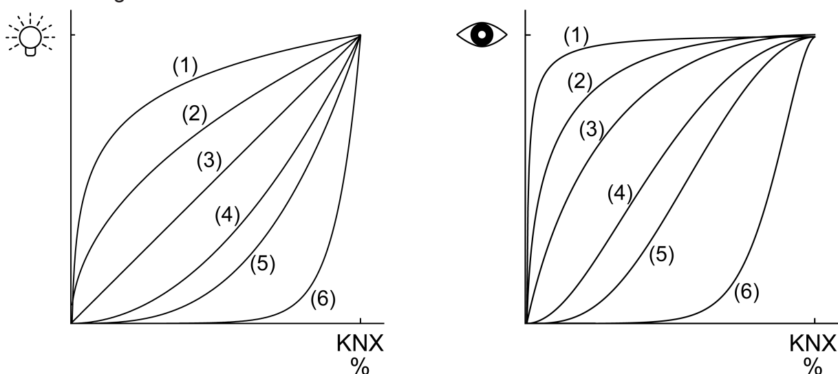
Figure 9: Dimming characteristics in the value range
