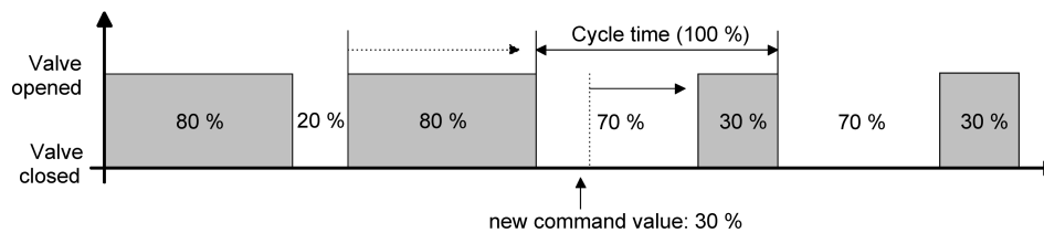
Figure 58: Example of a command value change 80% -> 30% during the closing phase of the valve
