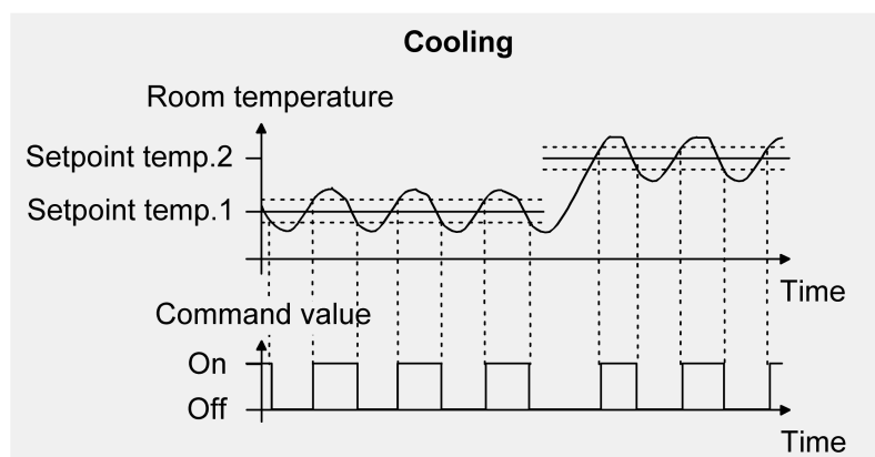
Figure 71: 2-point feedback control for the single "Cooling" operating mode
