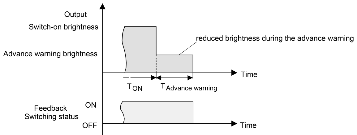
Figure 38: The pre-warning function of the staircase function without soft OFF function
