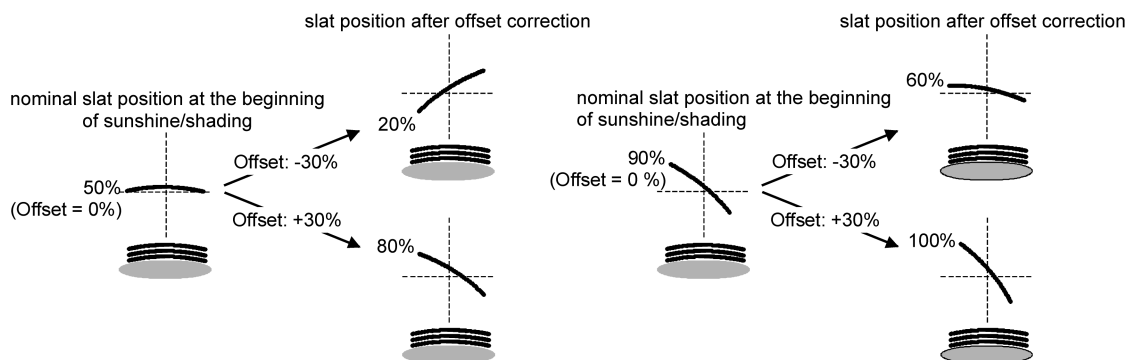
Figure 52: Functional principle of slat offset (example showing slat type 1 / slat type 2 identical)
