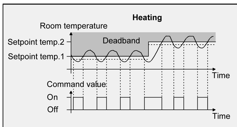
Figure 72: 2-point feedback control for mixed "Heating and cooling" mode with active heating mode
