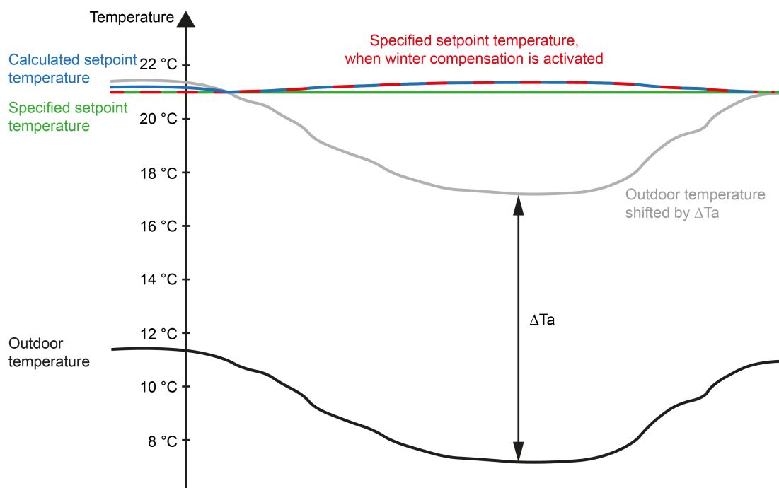
Figure 82: Example for winter compensation
