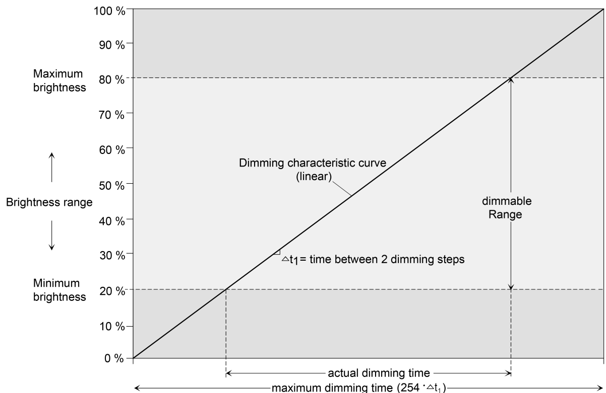
Figure 10: Linear characteristic dimming curve as an example with minimum brightness > 0 % and maximum brightness
