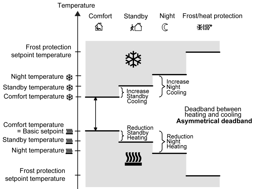
Figure 80: Setpoint temperatures in the operating mode "Heating and cooling" with asymmetrical deadband
