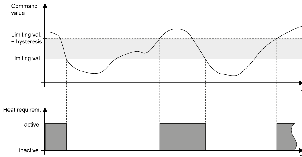
Figure 55: Heat requirement information with sample command value characteristic
