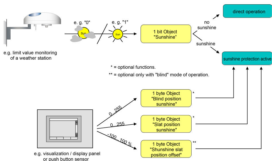
Figure 50: Schematic diagram illustrating of the sun protection configuration
