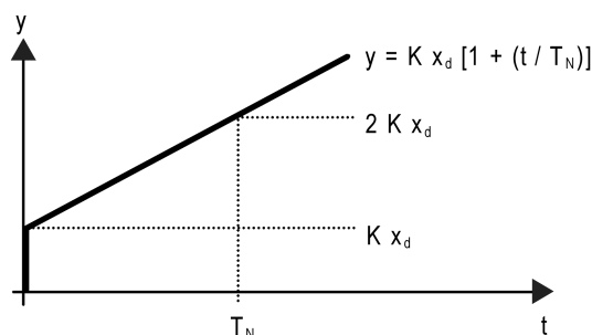
Figure 69: Function of the command value of a PI control
