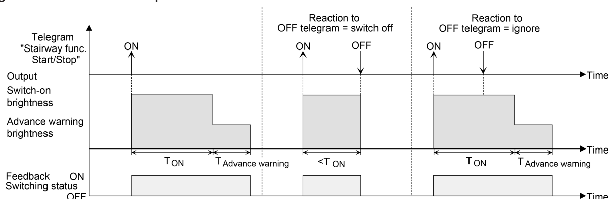
Figure 36: Switch-off behaviour of the staircase function without soft functions
