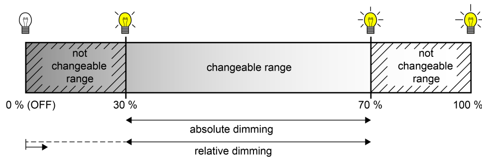
Figure 30: Example of a dimmable brightness range
