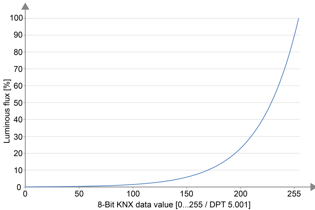
Figure 26: Logarithmic DALI dimming characteristic (relative luminous flux [%] depending on the 8-bit KNX data value [0...255])
