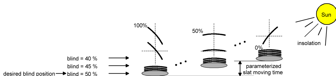
Figure 46: Example of slat positioning affecting the position of the Venetian blind (Typical of slat type 1; analogous reaction for type 2.)
