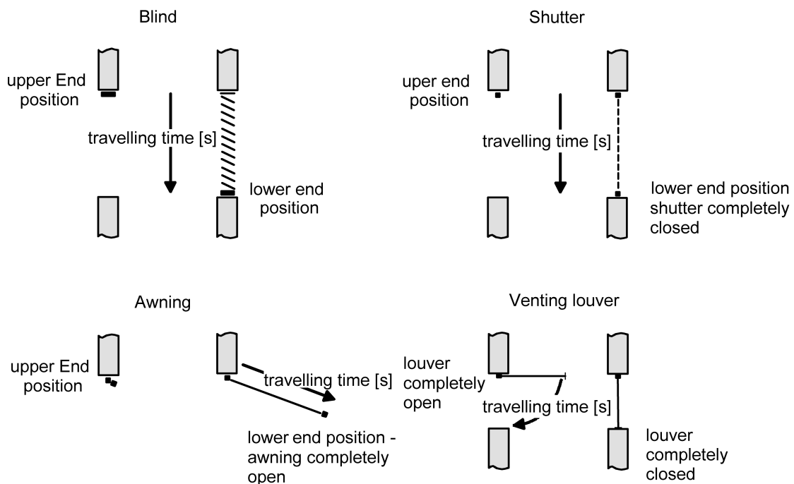
Figure 42: Determining the travel time according to the drive type
