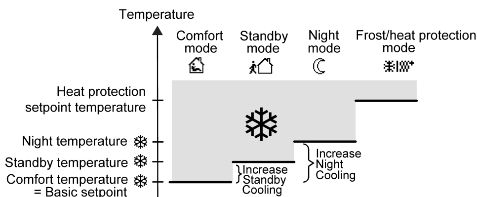
Figure 78: Setpoint temperatures in the operating mode "Cooling"
