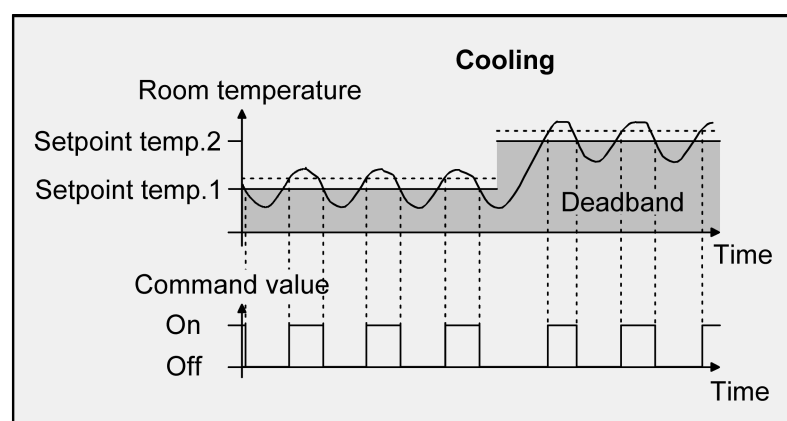
Figure 73: 2-point feedback control for mixed "Heating and cooling" mode with active cooling operation
