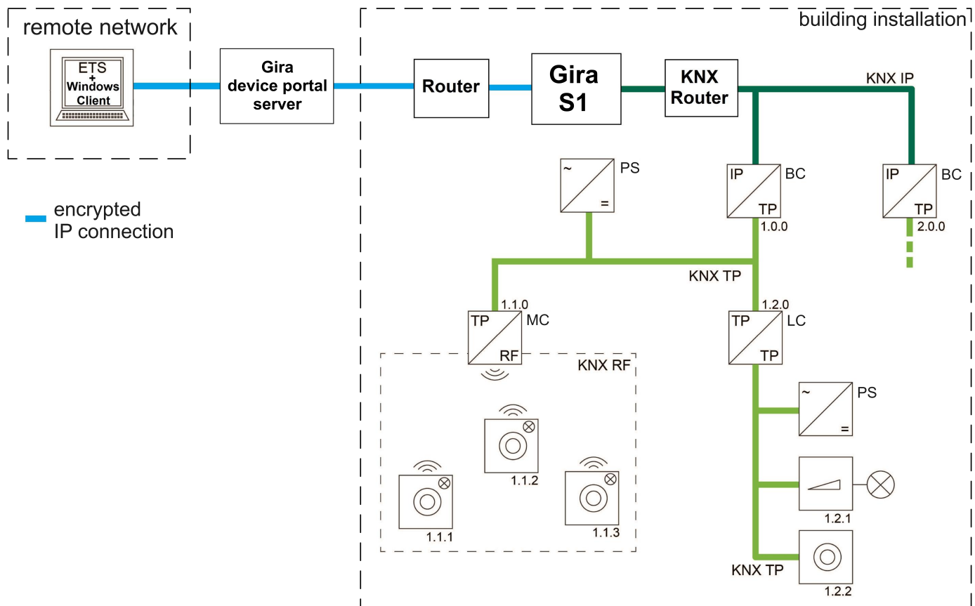
Figure 5: Possible KNX topology with a KNX IP connection of the ETS (KNX/net IP)
