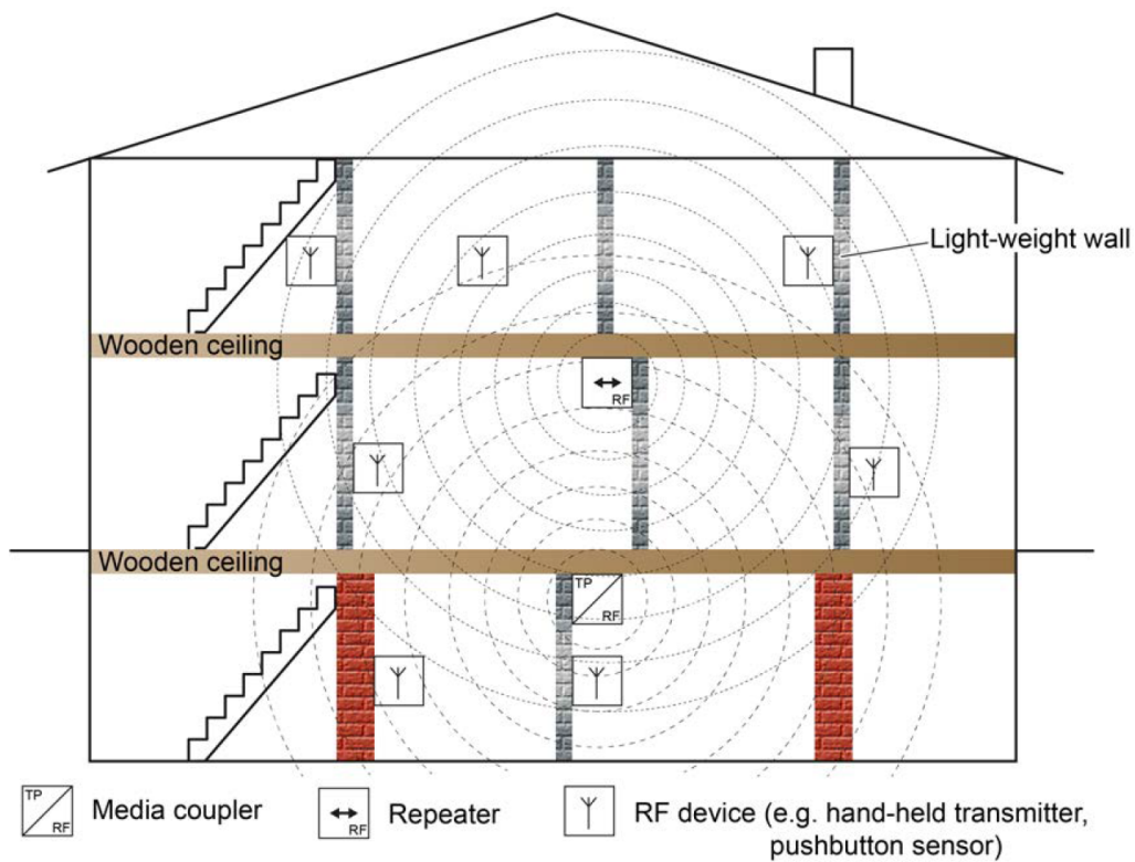
Figure 21: Building structure with a KNX RF line and repeater
