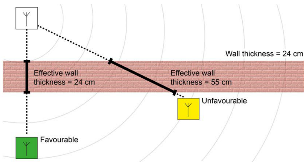
Figure 15: Attenuation through effective wall or ceiling thickness
