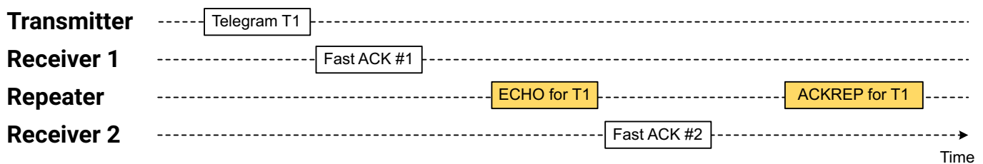
Figure 9: RF communication with repeater
