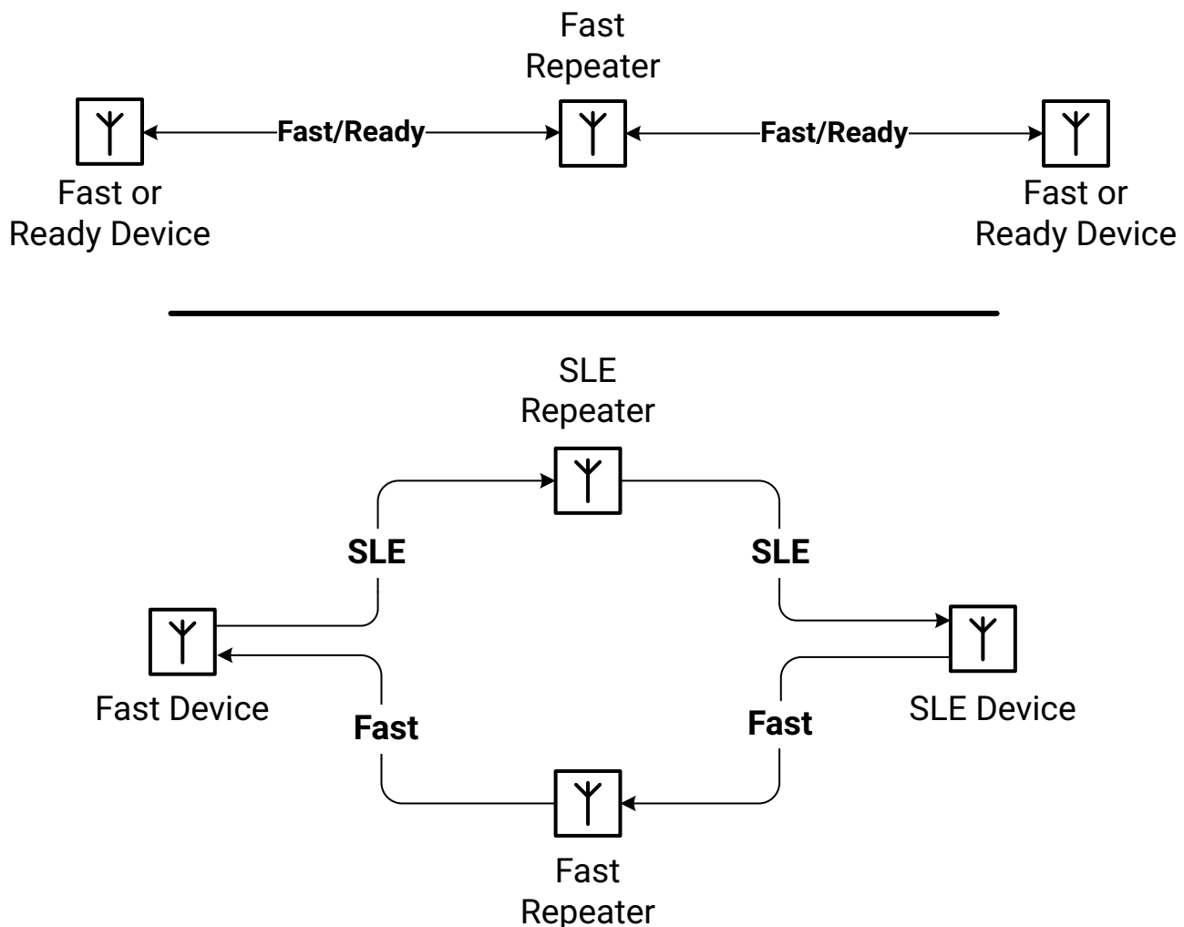
Figure 8: Difference between Fast/SLE repeater
