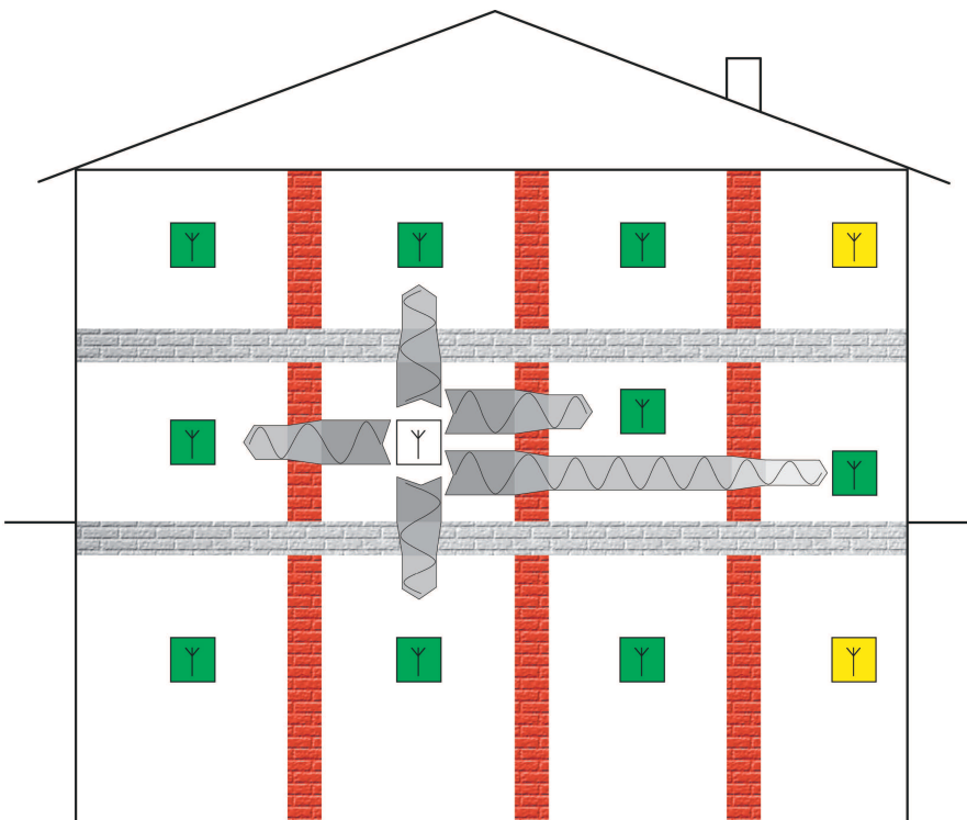
Figure 14: Attenuation of the radio signal by walls and ceilings (here: central position of the transmitter)
