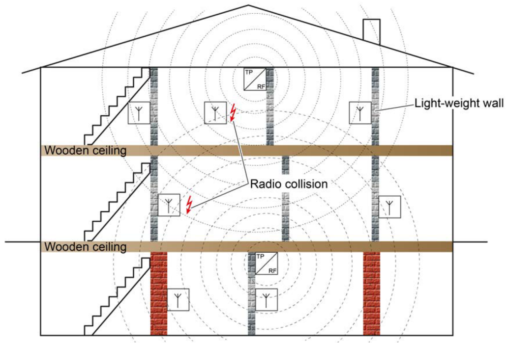
Figure 20: Building structure with two KNX RF lines, unfavourable interference
