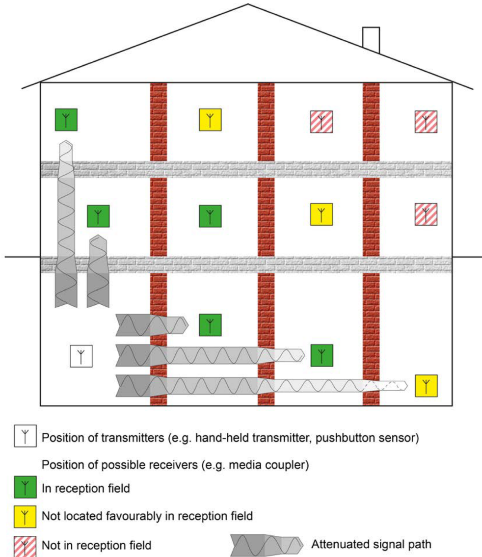
Figure 13: Attenuation of the radio signal by walls and ceilings (here: edge position of the transmitter)
