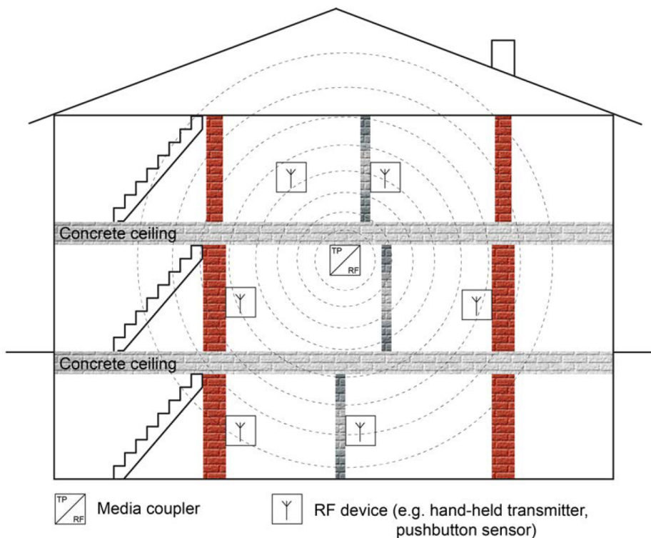
Figure 19: Building structure with a KNX RF line
